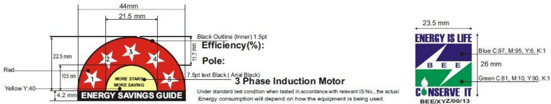
Figure 1: Design Scheme of Label(Sample)
